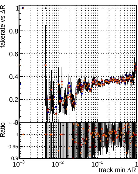
Fake rate vs \Delta R (track, jet) Legend: DOM mkFit (blue circles) DOM mkFit + T (orange circles) DOM mkFit + JanUpdate (red circles) Original (black line) JanUpdate (black line) statErr (black line) sysErr (black line)
