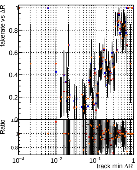
Fake rate vs \Delta R (track, jet) Legend: DOM mkFit T Original DOM mkFit T JanUpdate noErr DOM mkFit T JanUpdate statErr DOM mkFit T JanUpdate systErr
