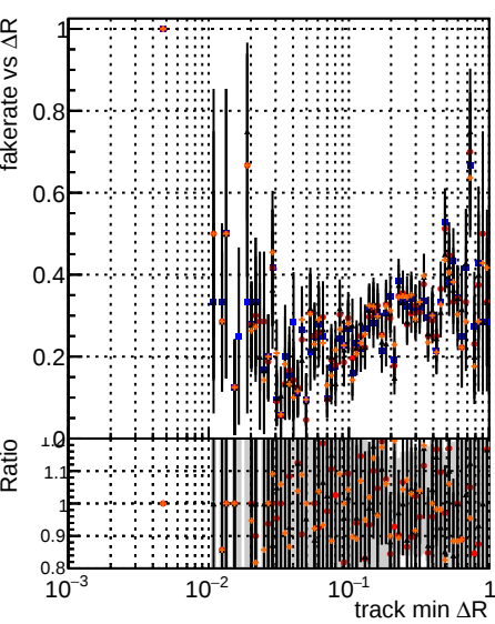
Fake rate vs \Delta R(\text{track, jet}) Legend: DOM mkFit DOM mkFit + T DOM mkFit + T + JanUpdate DOM mkFit + T + JanUpdate + noErr DOM mkFit + T + JanUpdate + statErr DOM mkFit + T + JanUpdate + systErr
