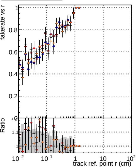
Fake rate vs v DOM mktFit TToriginal DOM mktFit JanUpdate-noErr DOM mktFit JanUpdate-statErr DOM mktFit JanUpdate-systErr
