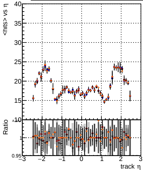
mean hit Legend: - DQM_mkFit_TT_Original (blue line with circles) - DQM_mkFit_TT_JanUpdate-noErr (red line with circles) - DQM_mkFit_TT_JanUpdate-statErr (black line with circles) - DQM_mkFit_TT_JanUpdate-systErr (orange line with circles)
