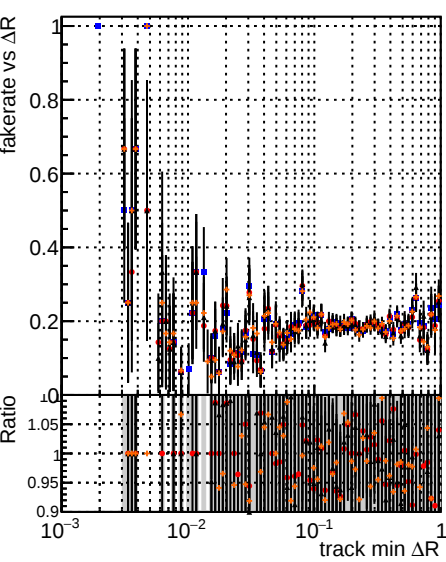
Fake rate vs \Delta R(\text{track, jet}) Legend: DOM mkFit TOriginal DOM mkFit JanUpdate-noErr DOM mkFit JanUpdate-statErr DOM mkFit JanUpdate-systErr
