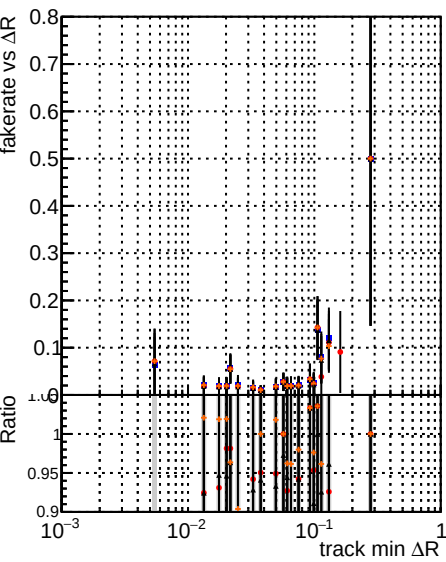
Fake rate vs ΔR(track, jet) Legend: DOM mktFit TtoOriginal DOM mktFit JanUpdate-noErr DOM mktFit JanUpdate-statErr DOM mktFit JanUpdate-systErr
