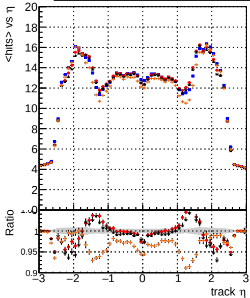
Legend: DQM_mkFit_TT_Original (blue line), DQM_mkFit_TT_JanUpdate-noErr (red line), DQM_mkFit_TT_JanUpdate-statErr (black line), DQM_mkFit_TT_JanUpdate-systErr (orange line) mean hit
