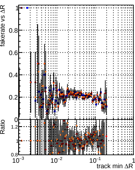
Fake rate vs \Delta R(\text{track, jet}) Legend: DOM mktFit TtoOriginal DOM mktFit JanUpdate-noErr DOM mktFit JanUpdate-statErr DOM mktFit JanUpdate-systErr
