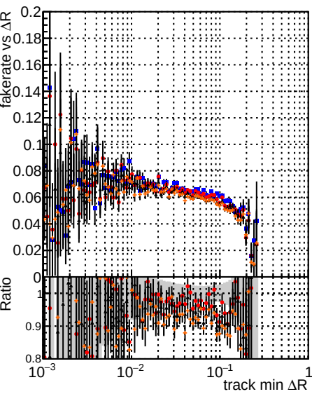
Fake rate vs \Delta R(\text{track, jet}) Legend: DOM mktFit T Original DOM mktFit T JanUpdate-noErr DOM mktFit T JanUpdate-statErr DOM mktFit T JanUpdate-systErr
