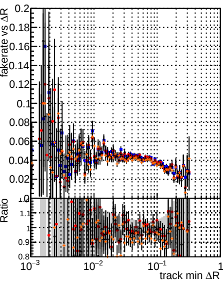
Fake rate vs \Delta R(\text{track}, \text{jet}) Legend: DOM mktFit T Original DOM mktFit T JanUpdate noErr DOM mktFit T JanUpdate statErr DOM mktFit T JanUpdate systErr
