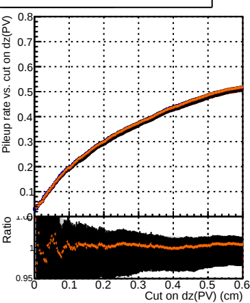
Pileup rate vs. cut on dz(PV) (cm)
