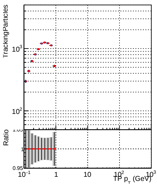
Legend: DQM_V0001_R000000001_Global_mkFit100Timeo_RECO (blue line with dots), DQM_V0001_R000000001_Global_mkFit100Timeo_RECO (red line with dots)
