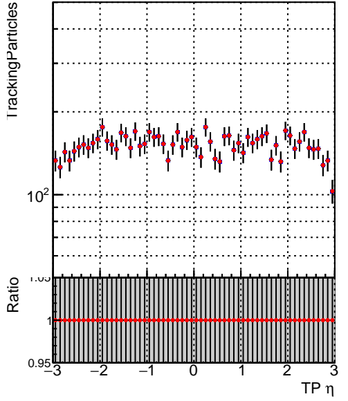
— DQM_V0001_R000000001_Global_mkFit100Timeo_RECO — DQM_V0001_R000000001_Global_mkFit100Timeo_RECO
