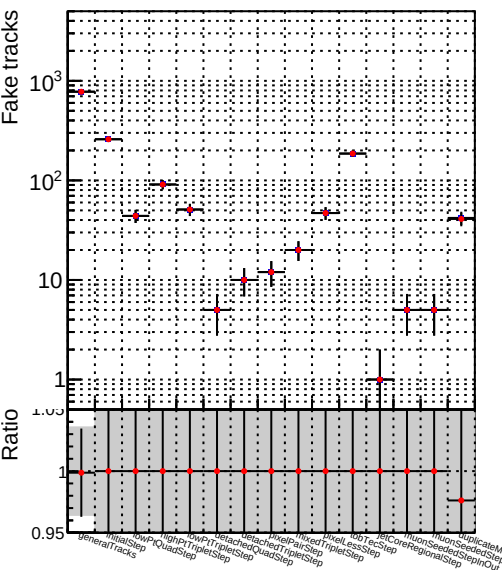
Number ● DQM_V0001_R000000001 Global mkFit100Time RECO
