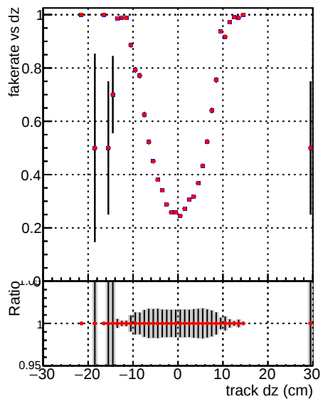
Fake rate vs dz — Global mkFit100Timeo RECO — Global mkFit100Time RECO
