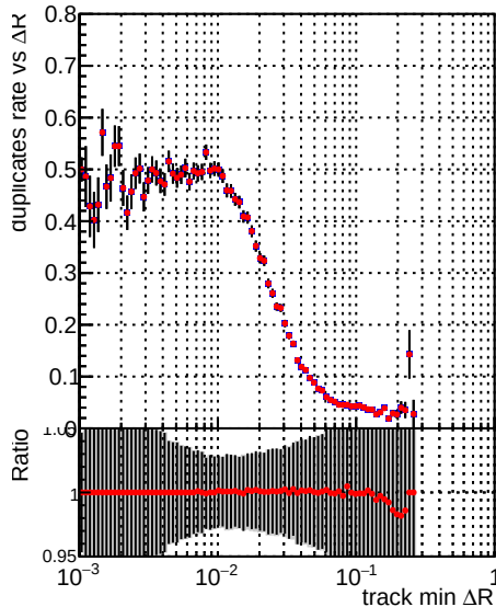
—•— DQM_V0001_R000000001_Global_mkFit100Timeo_RECO —•— DQM_V0001_R000000001_Global_mkFit100Time_RECO
