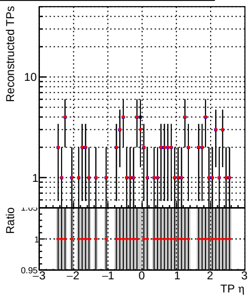
—•— DQM_V0001_R000000001_Global_mkFit100Timeo_RECO —•— DQM_V0001_R000000001_Global_mkFit100Time_RECO
