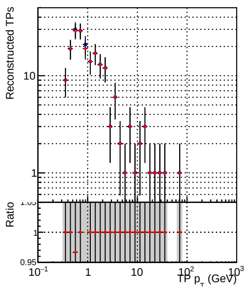
—•— DQM_V0001_R000000001_Global_mkFit100Timeo_RECO —•— DQM_V0001_R000000001_Global_mkFit100Time_RECO
