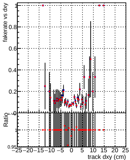
—●— DQM_V0001_R0000000001_Global_mkFit100Timeo_RECO —●— DQM_V0001_R0000000001_Global_mkFit100Timeo_RECO
