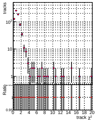
N of reco track vs. \chi^2 — Global_mkFit100Timeo_RECO — Global_mkFit100Timeo_RECO
