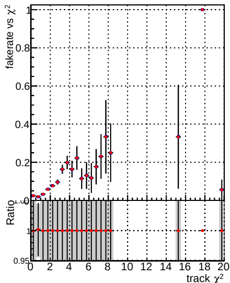
Fake rate vs. —●— DQM V0001_R000000001 Global mkFit100Timeo RECO —●— DQM V0001_R000000001 Global mkFit100Time RECO
