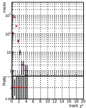
N of reco track vs. \chi^2 Global_mkFit100Time_RECO Global_mkFit100Time_RECO
