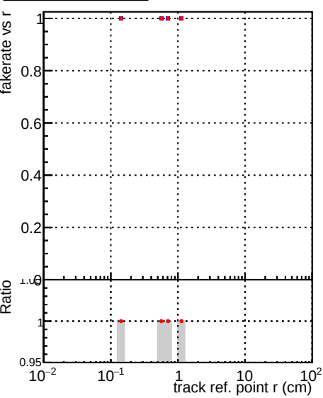
Legend: DQM_V0001_R000000001_Global_mkFit100Timeo_RECO (grey bars), DQM_V0001_R000000001_Global_mkFit100Time_RECO (red dots)
