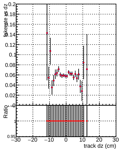
Legend Global mkFit100Timeo RECO Fake rate vs d Blue line with dots Global mkFit100Timeo RECO Red line with dots Global mkFit100Time RECO
