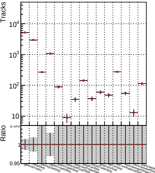
DQM_V0001_R0000000001_Global_mkFit100Timeo_RECO
