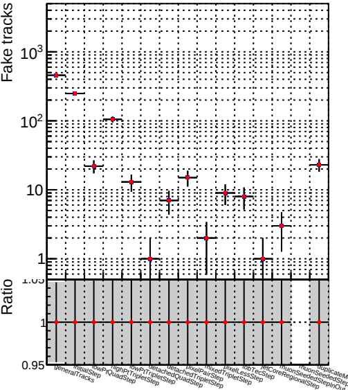
Number ● DQM_V0001_R000000001_Global_mkFit100Time_RECO
