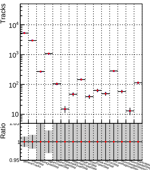
■ DQM_V0001_R0000000001_Global_mkFit100Timeo_RECO
