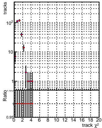
N of reco track vs. \chi^2 for DQM_V0001_R000000001_Global_mkFit100Timeo_RECO and DQM_V0001_R000000001_Global_mkFit100Timeo_RECO
