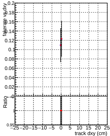
—•— DQM_V0001_R0000000001_Global_mkFit100Timeo_RECO —•— DQM_V0001_R0000000001_Global_mkFit100Timeo_RECO
