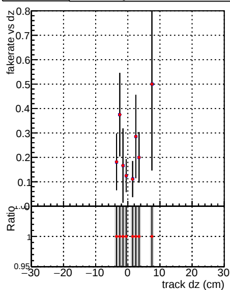
—•— DQM_V0001_R0000000001_Global_mkFit100Timeo_RECO —•— DQM_V0001_R0000000001_Global_mkFit100Timeo_RECO
