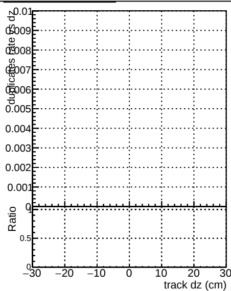
—•— DQM_V0001_R0000000001_Global_mkFit100Timeo_RECO —•— DQM_V0001_R0000000001_Global_mkFit100Timeo_RECO
