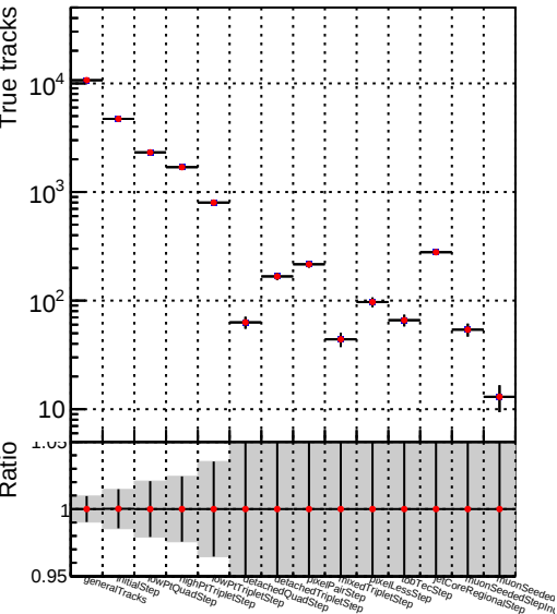
DQM_V0001_R000000001_Global_mkFit100Timeo__RECO
