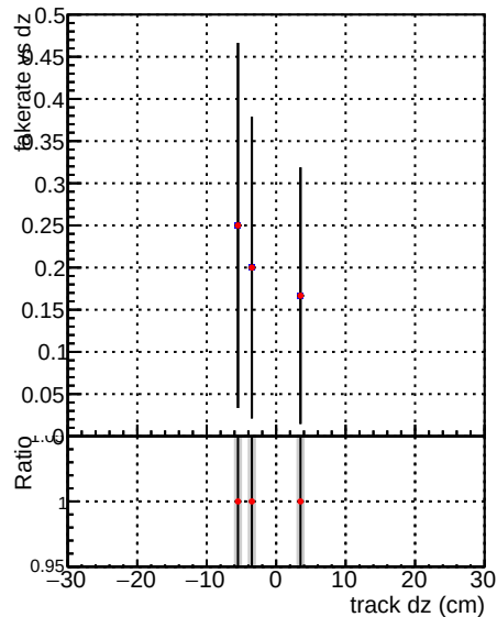
Global mkFit100Timeo RECO —●— DQM V0001_R000000001 —●— DQM V0001_R000000001
