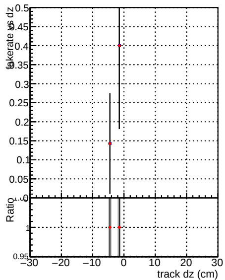
█ █ DQM_V0001_R0000000001_Global_mkFit100Timeo_RECO █ █ DQM_V0001_R0000000001_Global_mkFit100Time_RECO
