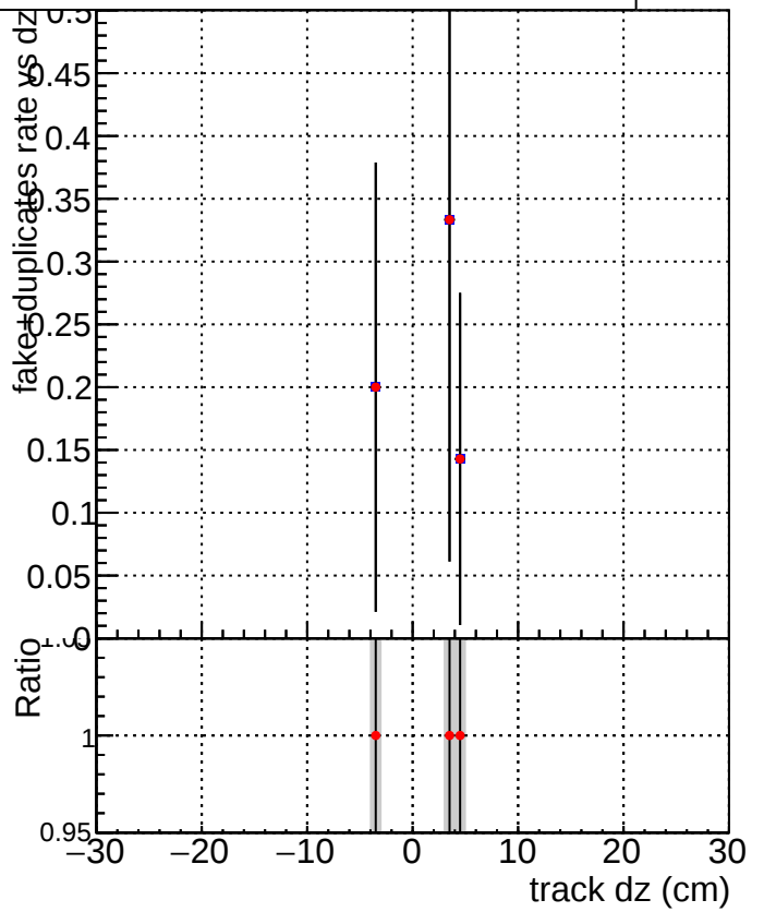
DQM_V0001_R0000000001_Global_mkFit100Timeo_RECO DQM_V0001_R0000000001_Global_mkFit100Time_RECO
