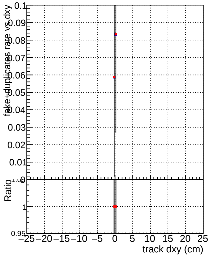
DQM_V0001_R0000000001_Global_mkFit100Timeo_RECO DQM_V0001_R0000000001_Global_mkFit100Time_RECO
