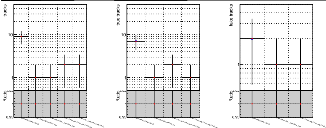
N of reco track vs. \chi^2 DQM_V0001_R0000000001_Global_mkFit100Timeo_RECO DQM_V0001_R0000000001_Global_mkFit100Timeo_RECO
