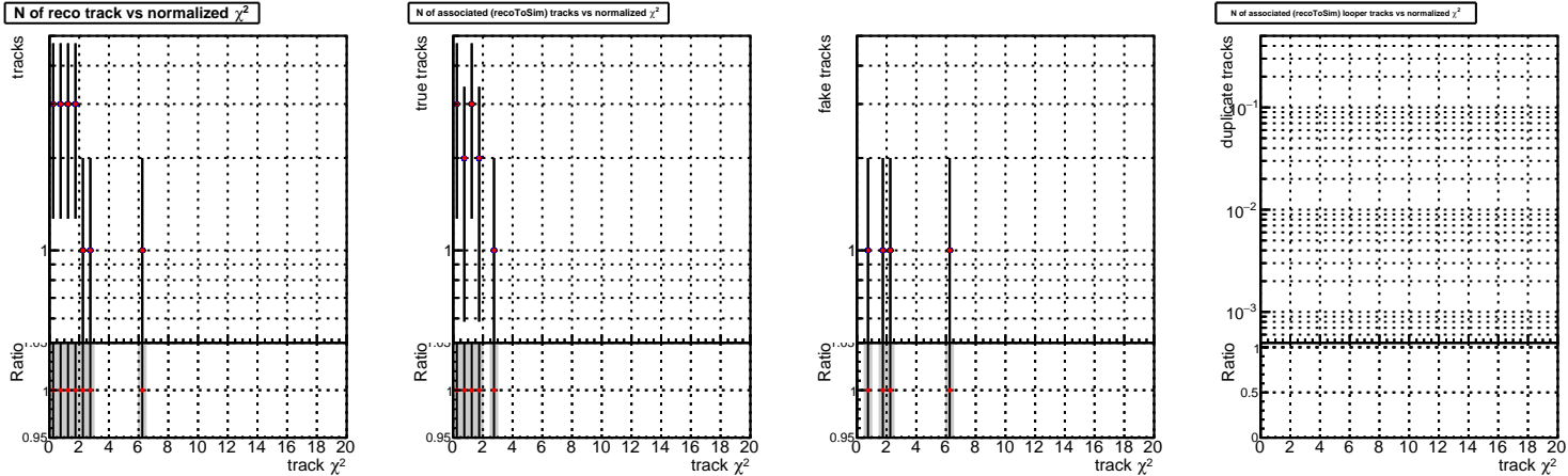
N of reco track vs. \chi^2 DQM_V0001_R0000000001_Global_mkFit100Timeo_RECO DQM_V0001_R0000000001_Global_mkFit100Timeo_RECO
