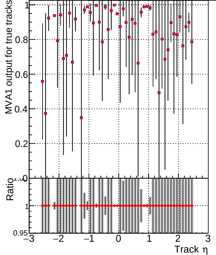
MVA1 of associated tracks (recoToSim) vs. track \eta Legend: ■ DQM_V0001_R000000001_Global_mkFit100Timeo_RECO ● DQM_V0001_R000000001_Global_mkFit100Time_RECO
