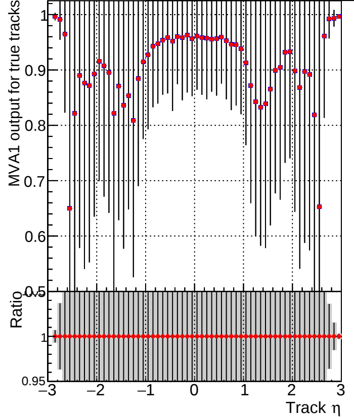
MVA1 of associated tracks (recoToSim) vs. track \eta ■ DQM_V0001_R000000001_Global_mkFit100Timeo_RECO ● DQM_V0001_R000000001_Global_mkFit100Time_RECO
