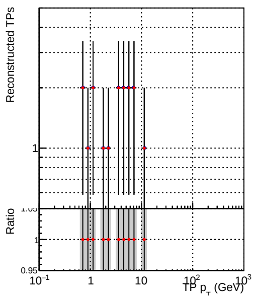
— DQM_V0001_R0000000001_Global_mkFit100Time_RECO — DQM_V0001_R0000000001_Global_mkFit100Time_RECO
