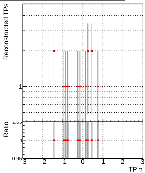
— DQM_V0001_R0000000001_Global_mkFit100Time_RECO — DQM_V0001_R0000000001_Global_mkFit100Time_RECO
