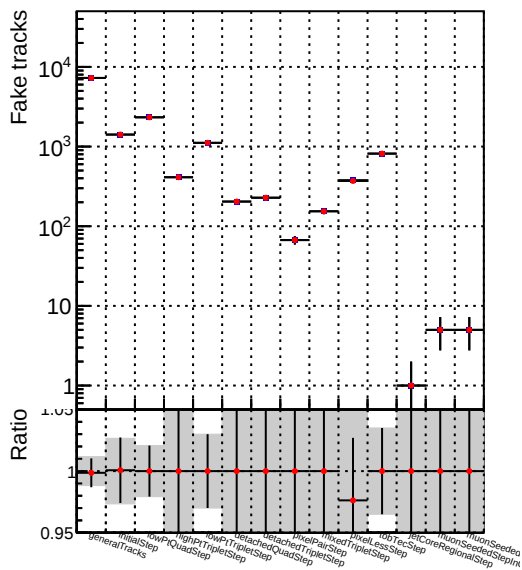
Number ● DQM_V0001_R000000001_Global_mkFit100Time_RECO
