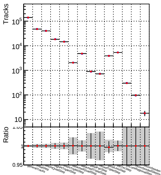
DQM_V0001_R000000001__Global__mkFit100Timeo__RECO
