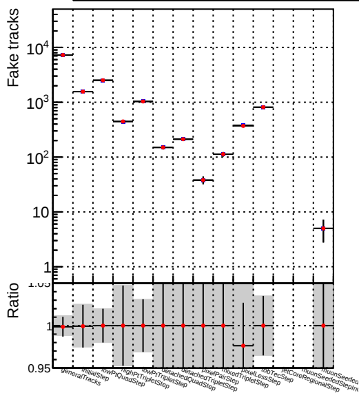
Number ● DQM_V0001_R0000000001_Global_mkFit100Time_RECO
