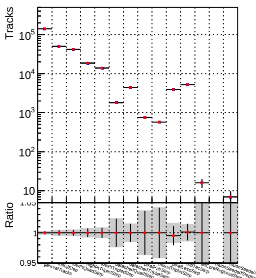
DQM_V0001_R000000001_Global_mkFit100Timeo_RECO
