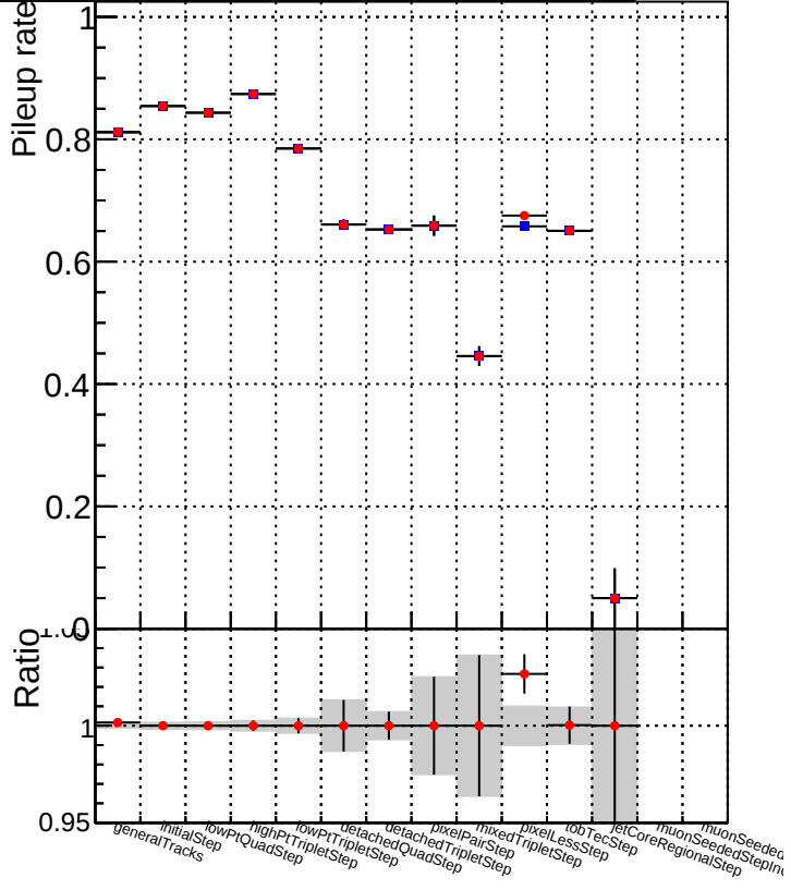
DQM_V0001_R0000000001_Global_mkFit100Timeo_RECO
