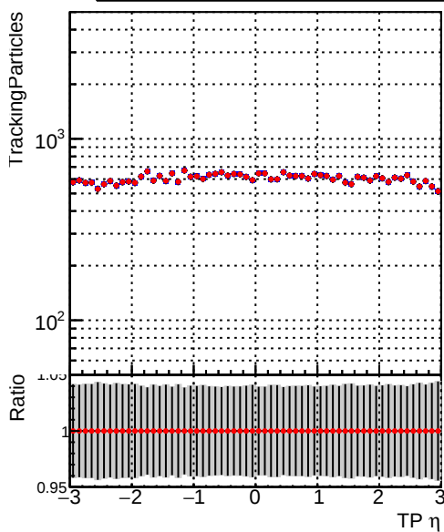
N of simulated tracks vs \eta DQM_V0001_R000000001_Global_mkFit100Timeo_RECO DQM_V0001_R000000001_Global_mkFit100Timeo_RECO
