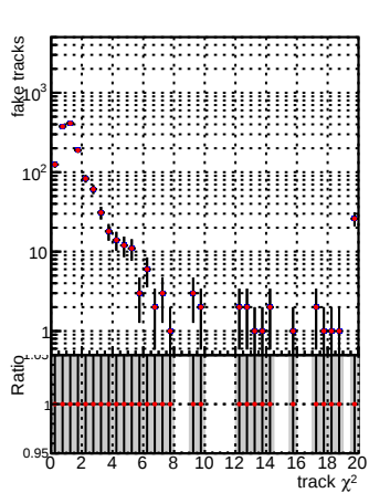
N of reco track vs. —●— DOM_V0001_R000000001_Global_mkFit100timeo_RECO —●— DOM_V0001_R000000001_Global_mkFit100timeo_RECO verSet
