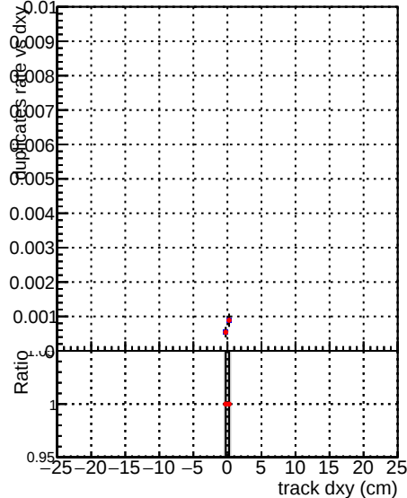
—•— DQM_V0001_R0000000001_Global_mkFit100Timeo_RECO —•— DQM_V0001_R0000000001_Global_mkFit100Time_RECO
