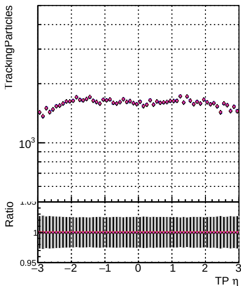
DOM V0001 R0000000001 Global mkFit1000 RECO N of sim DOM V0001 R0000000001 Global mkFit1000 RECO DOM V0001 R0000000001 Global mkFit1000 RECO DOM V0001 R0000000001 Global mkFit1000ATime RECO DOM V0001 R0000000001 Global mkFit1000CTime RECO DOM V0001 R0000000001 Global mkFit1000MTTime RECO
