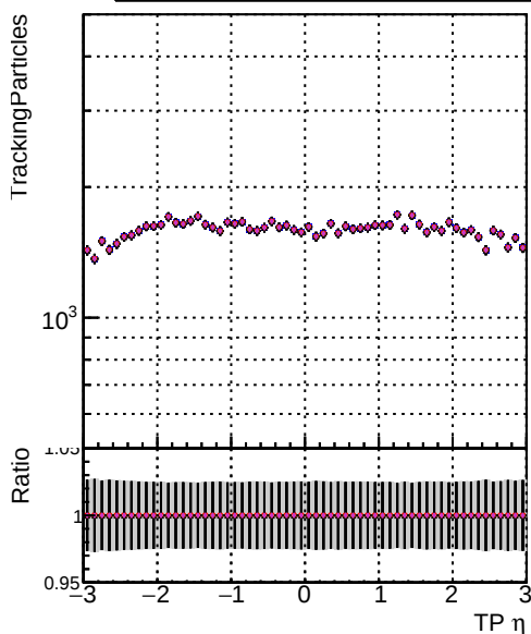
N of sim Model Model ID Model Name Model Type Model Description Model Status 1 DOM V0001 R0000000001 Global mkFit1000ATime RECO 2 DOM V0001 R0000000001 Global mkFit1000CTime RECO 3 DOM V0001 R0000000001 Global mkFit1000MTime RECO
