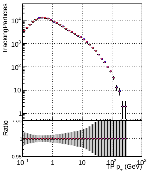
N of simulated tracks vs pT 0 1000 1 1000 2 1000 3 1000 4 1000 5 1000 6 1000 7 1000 8 1000 9 1000 10 1000 11 1000 12 1000 13 1000 14 1000 15 1000 16 1000 17 1000 18 1000 19 1000 20 1000 21 1000 22 1000 23 1000 24 1000 25 1000 26 1000 27 1000 28 1000 29 1000 30 1000 31 1000 32 1000 33 1000 34 1000 35 1000 36 1000 37 1000 38 1000 39 1000 40 1000 41 1000 42 1000 43 1000 44 1000 45 1000 46 1000 47 1000 48 1000 49 1000 50 1000 51 1000 52 1000 53 1000 54 1000 55 1000 56 1000 57 1000 58 1000 59 1000 60 1000 61 1000 62 1000 63 1000 64 1000 65 1000 66 1000 67 1000 68 1000 69 1000 70 1000 71 1000 72 1000 73 1000 74 1000 75 1000 76 1000 77 1000 78 1000 79 1000 80 1000 81 1000 82 1000 83 1000 84 1000 85 1000 86 1000 87 1000 88 1000 89 1000 90 1000 91 1000 92 1000 93 1000 94 1000 95 1000 96 1000 97 1000 98 1000 99 1000 100 1000
