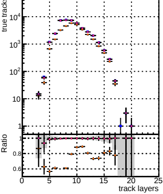
N of associated (recoToSim) tracks vs track layers
