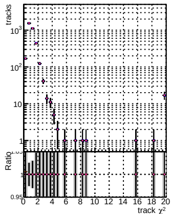
N of reco track vs. BSM V0001 R0000000001 Global mFit10000-RECO BSM V0001 R0000000001 Global mFit10000-ATLAS RECO
