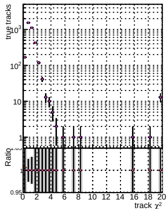
N of reco track vs. BSM V0001 R0000000001 Global mFit10000-RECO BSM V0001 R0000000001 Global mFit10000-ATLAS RECO
