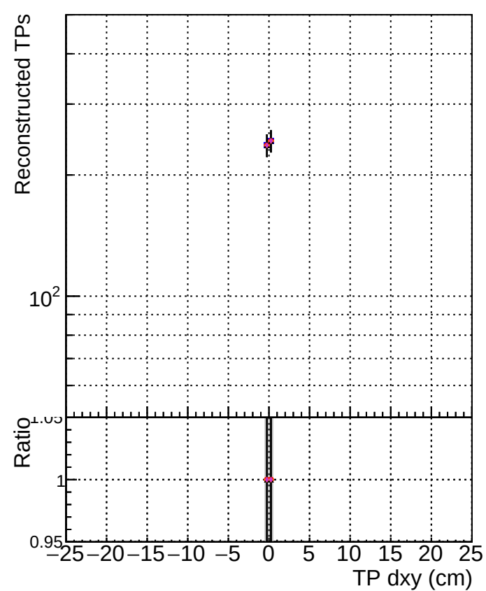
N of simulated track DOM_V0001 R000000001 Global mkFit1000o RECO DOM_V0001 R000000001 Global mkFit1000 RECO DOM_V0001 R000000001 Global mkFit1000ATime RECO DOM_V0001 R000000001 Global mkFit1000CTime RECO DOM_V0001 R000000001 Global mkFit1000MTime RECO
