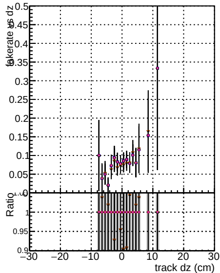
Fake rate vs d DOM V00001 P00000000000001 G00000000000000 m0000110000 P00000000000000
